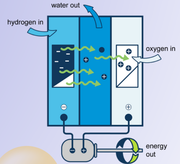
Hydrogen fuel cell
